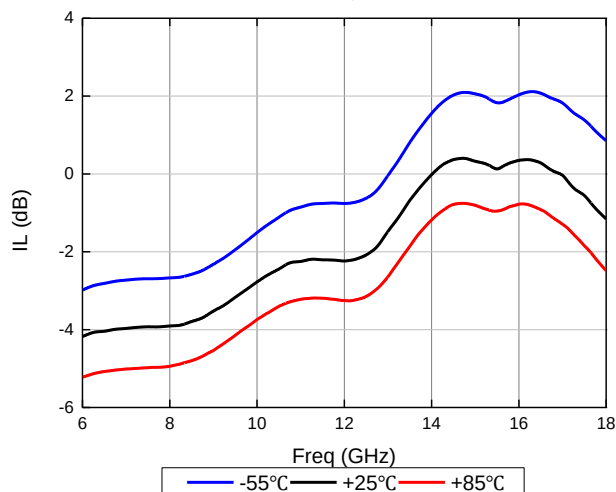
插入损耗
