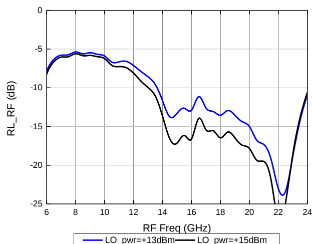
射频回波损耗 (IF=0.1GHz)
