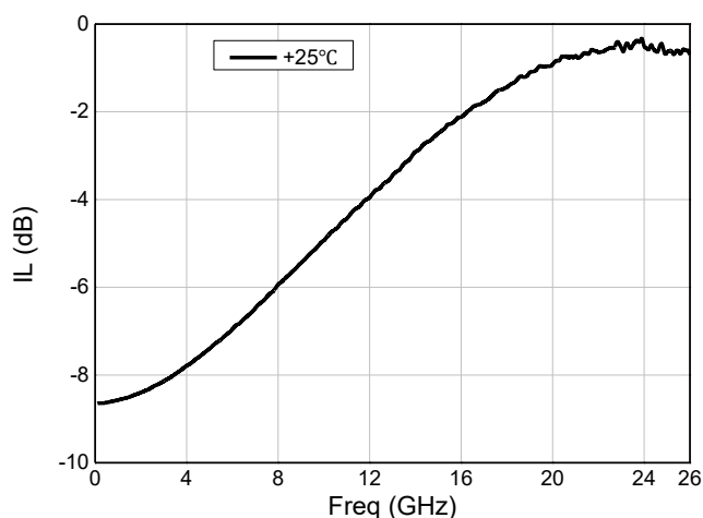
插入损耗
