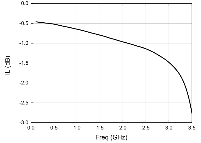
插入损耗
