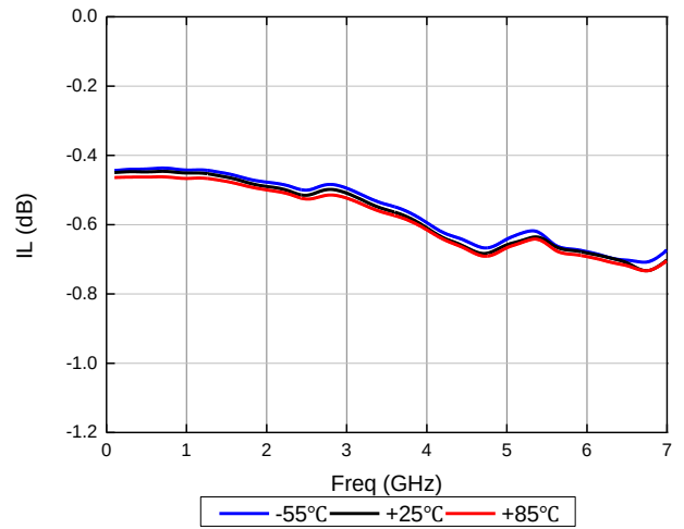
RFC-RF2插入损耗
