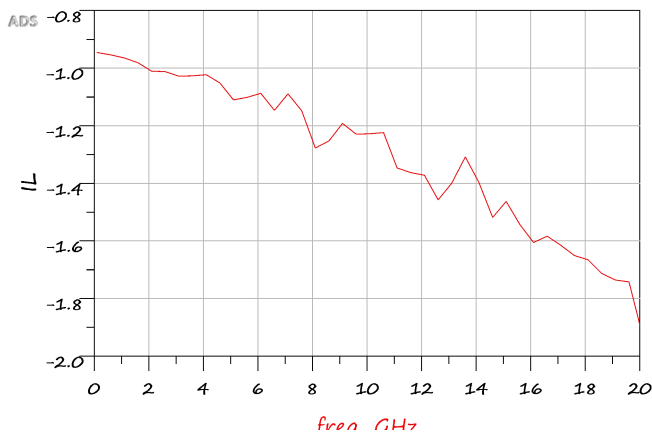
插入损耗
